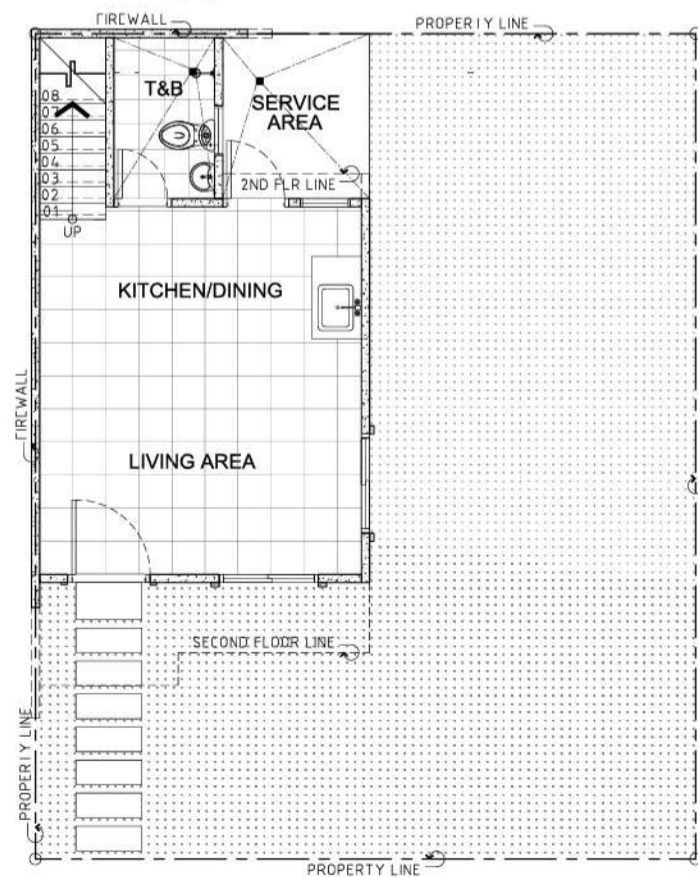
Typical First Floor Plan
