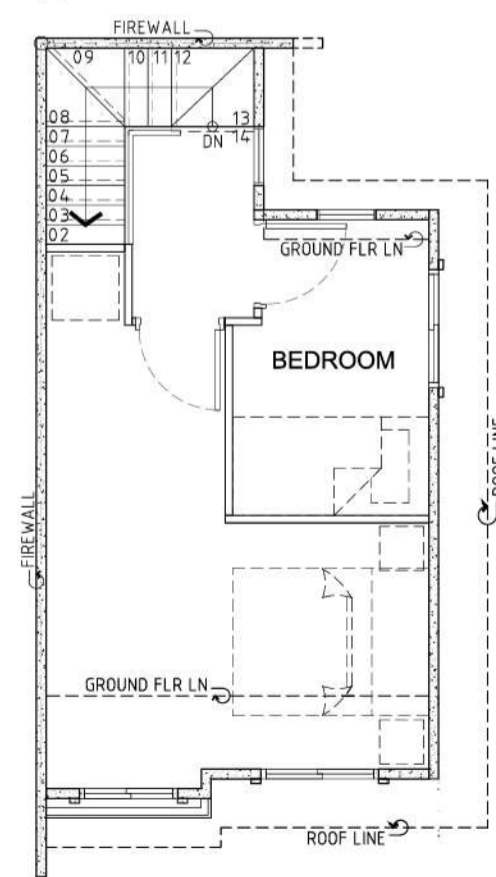
Typical Second Floor Plan
