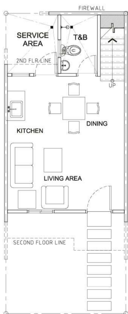
Typical First Floor Plan Typical Second Floor Plan
